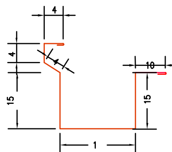
10. Jgheab metalic
