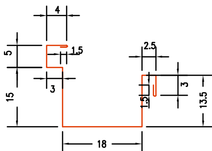
9. Jgheab metalic
