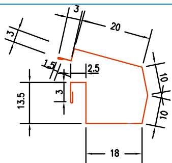
7. Jgheab metalic
